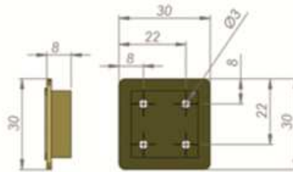
Wall fitting for calculator
