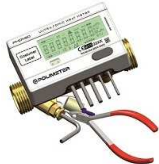
Brass body seal
